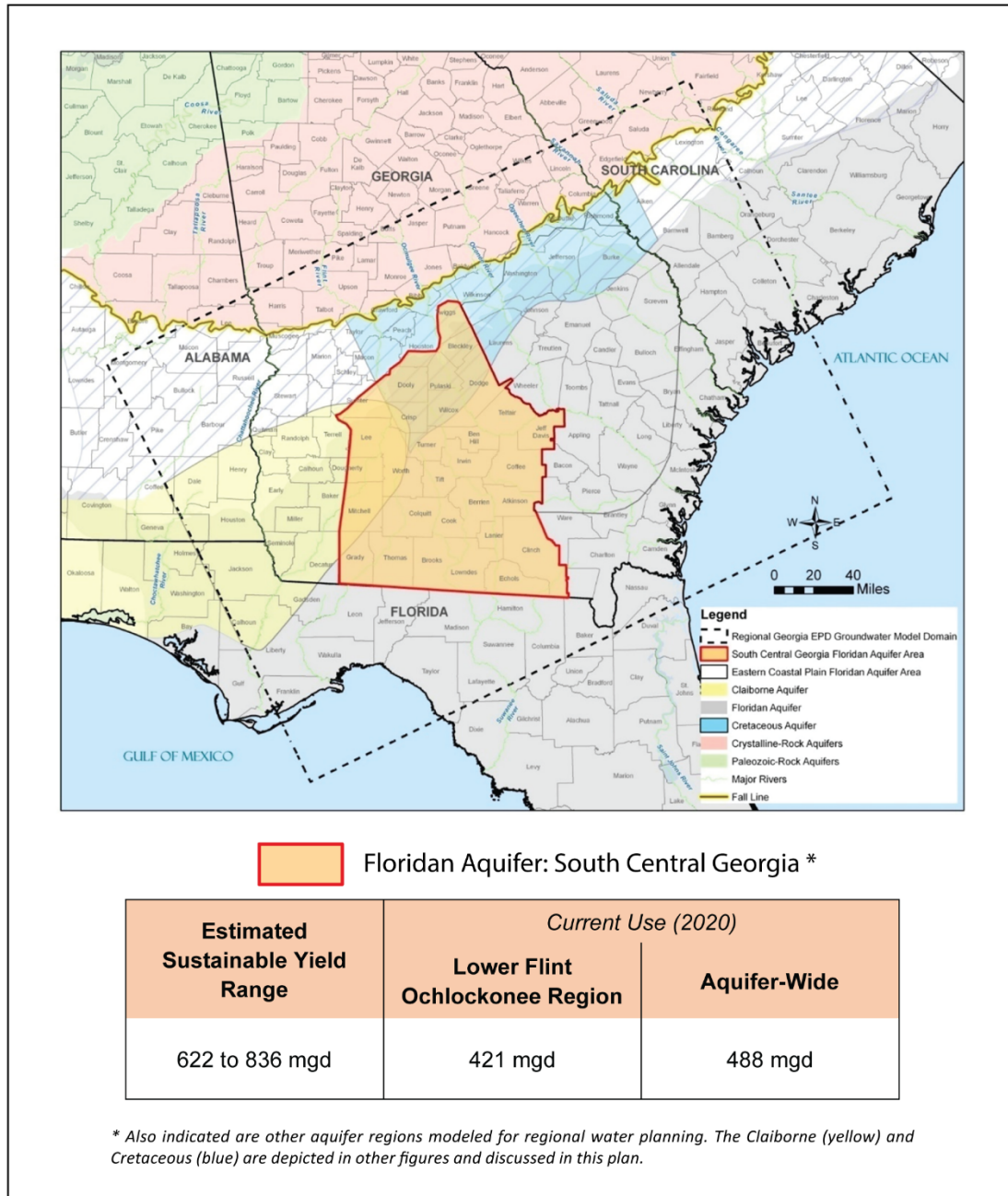
Figure 3-5: Floridan Aquifer: South Central Georgia – Model Domain and Estimated Sustainable Yield Range
