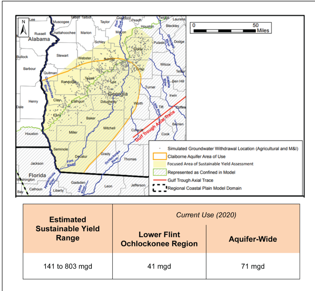
Figure 3-10: Claiborne Aquifer – Model Domain and Sustainable Yield
