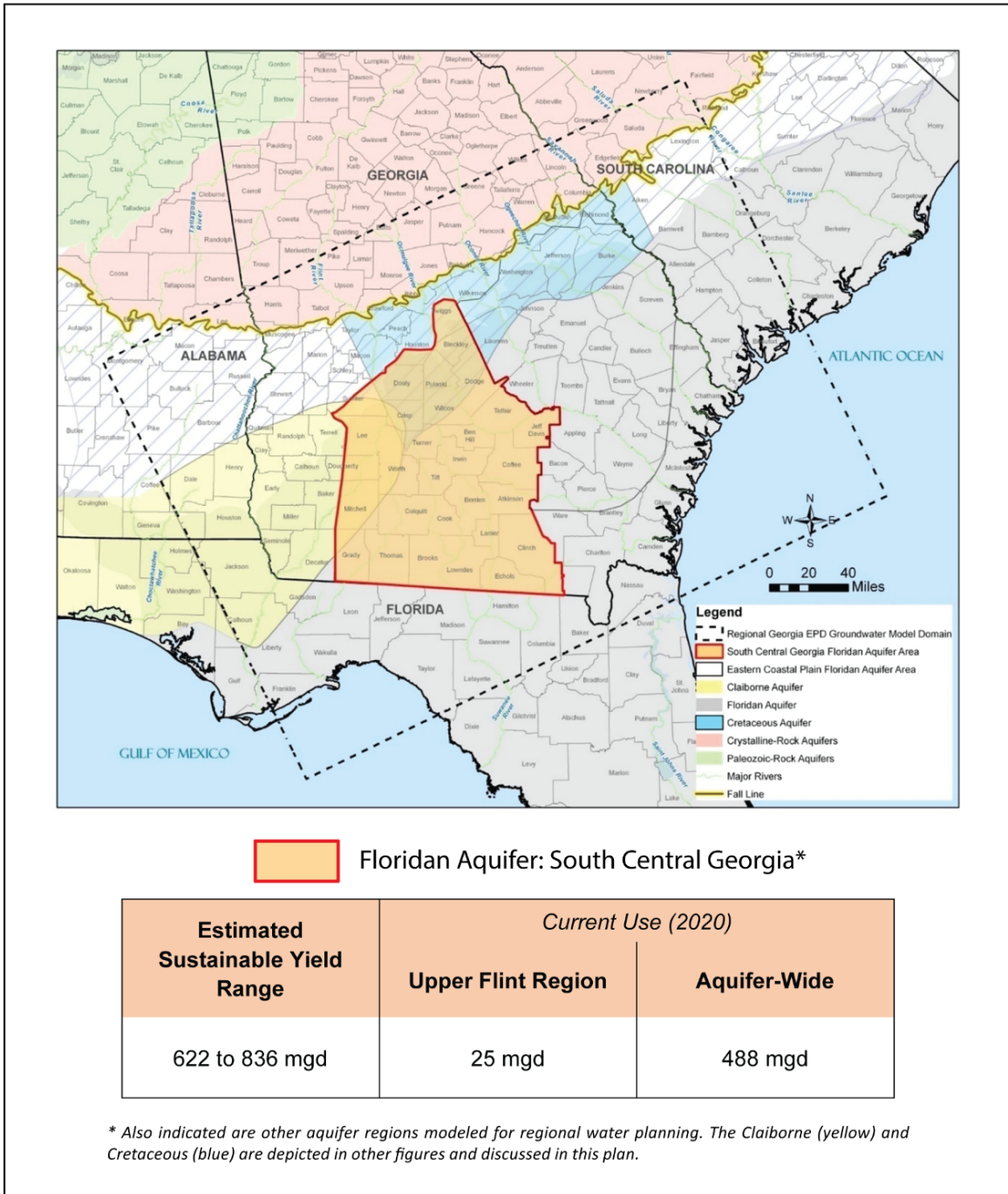
Figure 3-5: Floridan Aquifer: South-Central Georgia – Model Domain and Sustainable Yield
