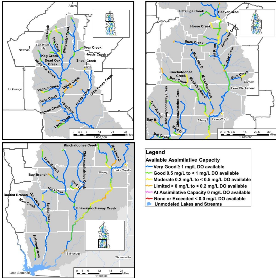
Figure 5-1: Assimilative Capacity Results from Dissolved Oxygen Assessment: Flint Basin (2050)
