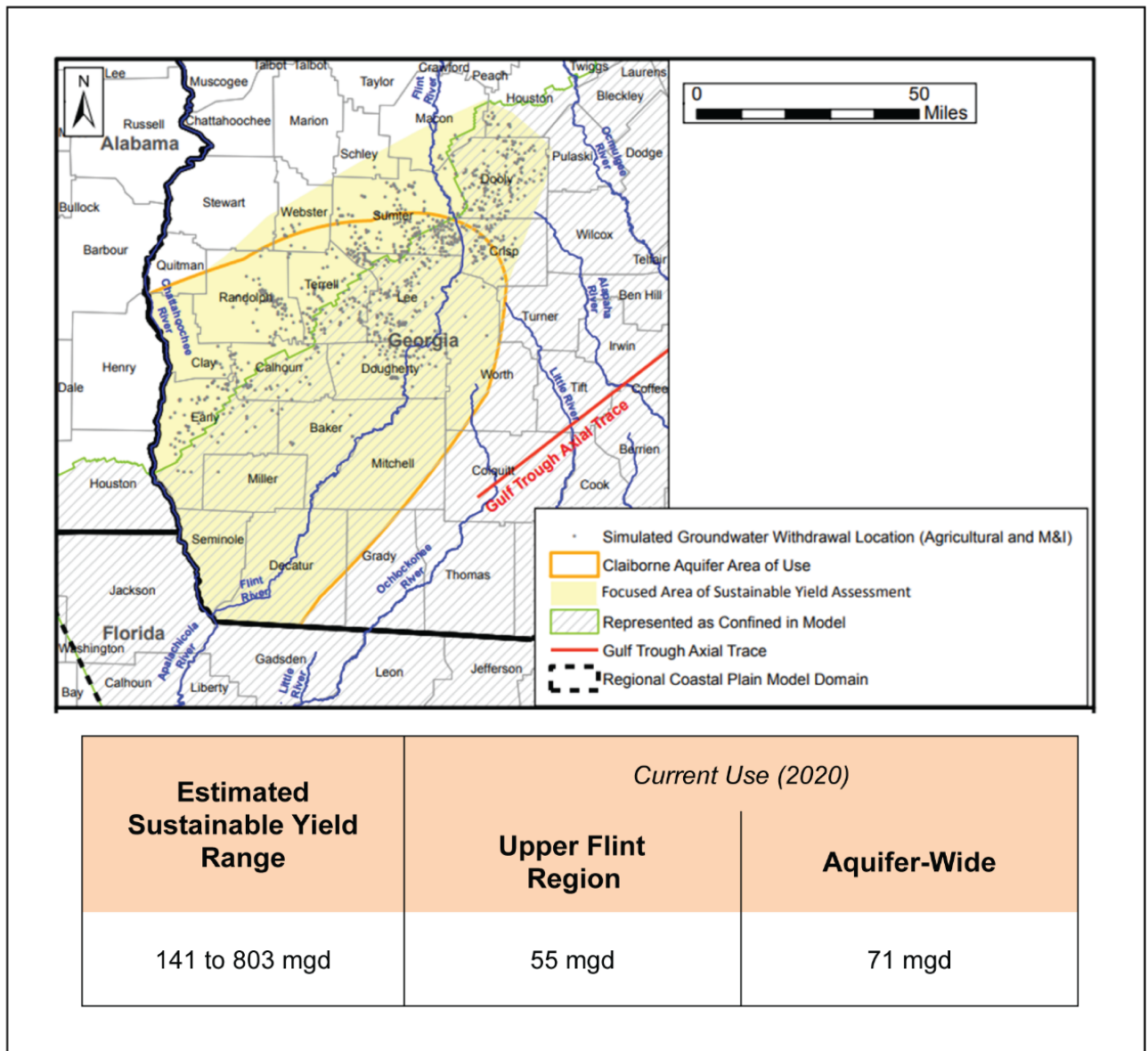
Figure 3-11: Claiborne Aquifer – Model Domain and Sustainable Yield
