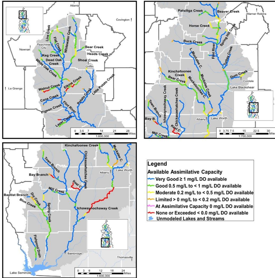
Figure 3-12: Assimilative Capacity Results from Dissolved Oxygen Assessment: Flint River Basin (Current)
