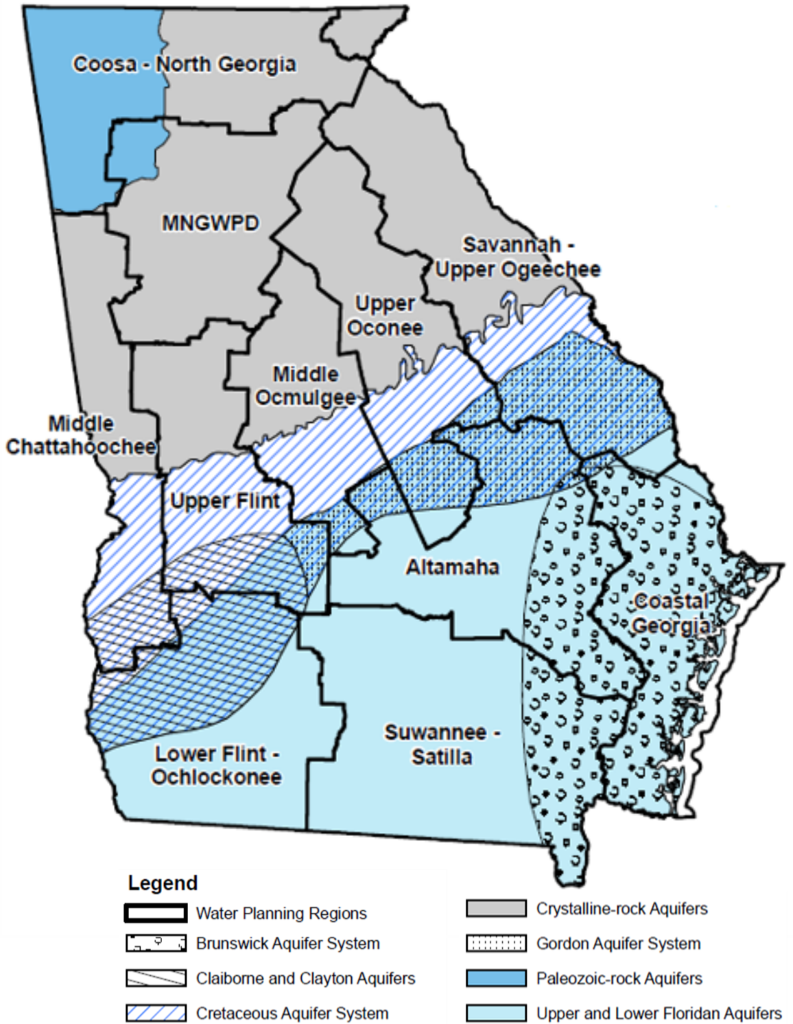
Figure 3-3: Georgia's Aquifers
